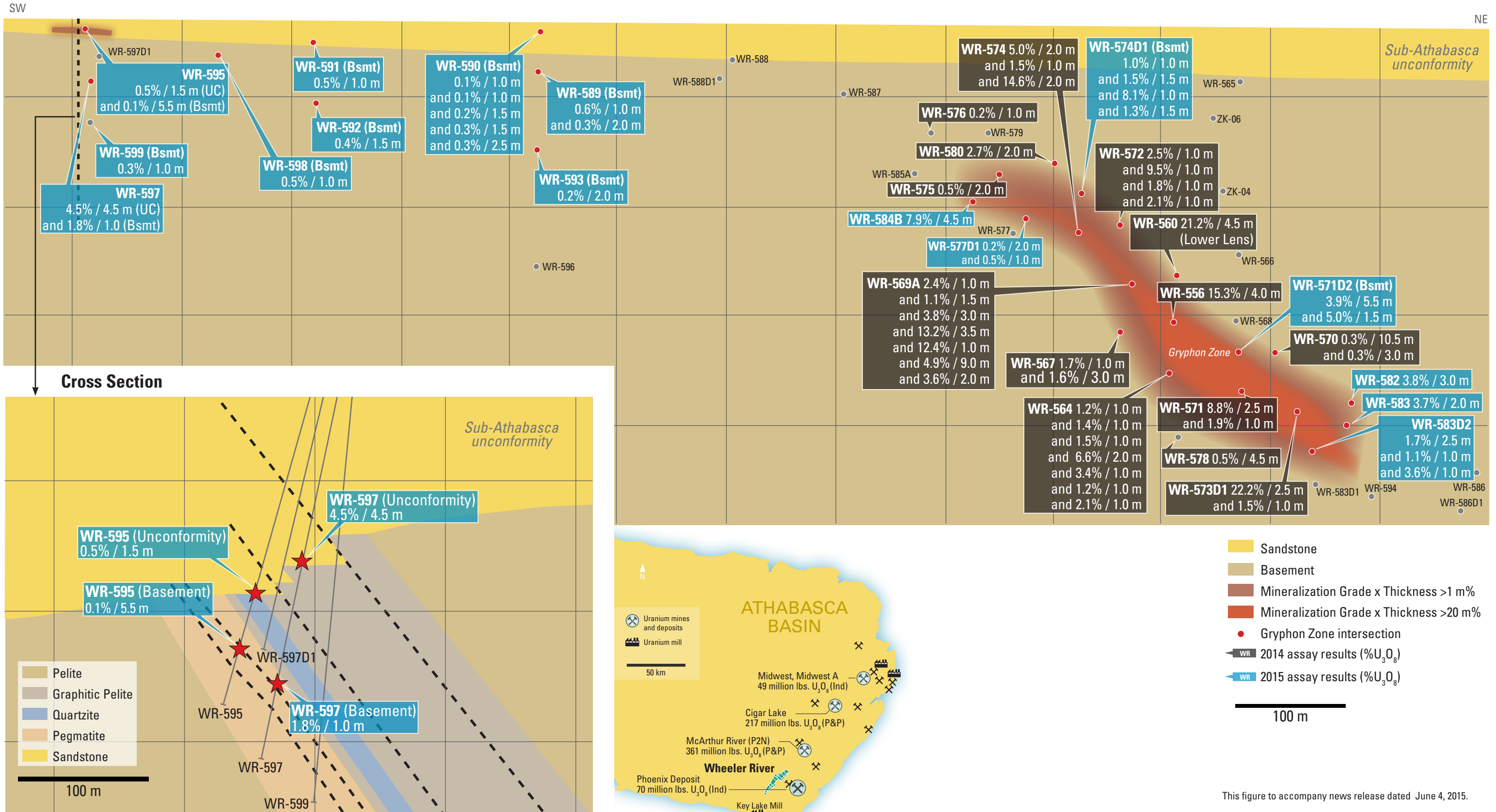
Gryphon Zone Upper Lens Inclined Longitudinal Section (Oriented 015/45E) June 4, 2015
